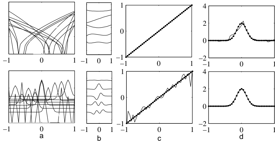
FIGURE 5.1. Top: Monotonic, broadly tuned population. Bottom: Gaussian-tuned population. (a) Tuning Curves. (b) First five \chi_i(x) 's. (c) Decoding results for f(x) = x . (d) Decoding results for a localized function f(x) . Dotted line is the desired function; solid line is the actual result. For (a),(c),and (d), N=20 . For (b), N=200 .
