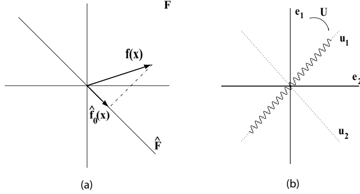
FIGURE 3.1. (a) Projection theorem Geometry. (b) Statespace rotation.
