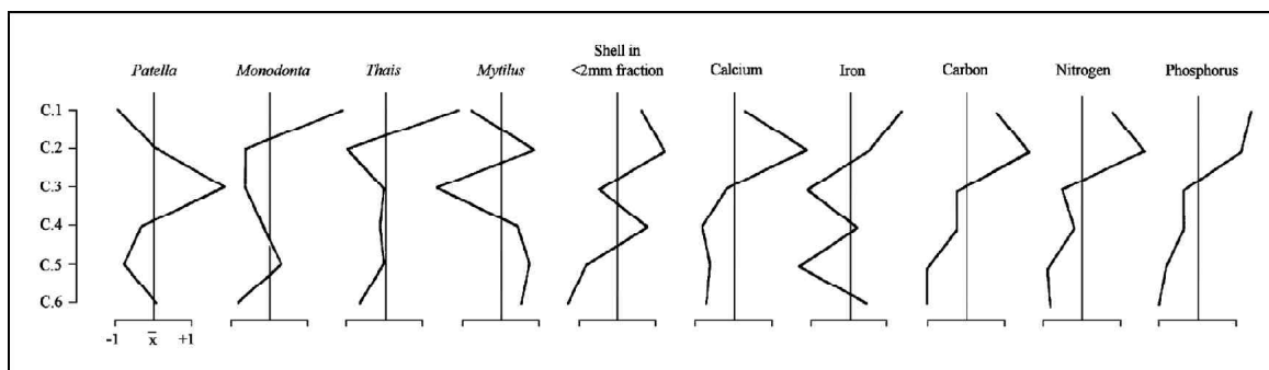
FIGURE 2. Summary of faunal and geochemical analyses of the Medo Tojeiro shell midden using Z scores (deviation around the mean). For description of levels, see text.
